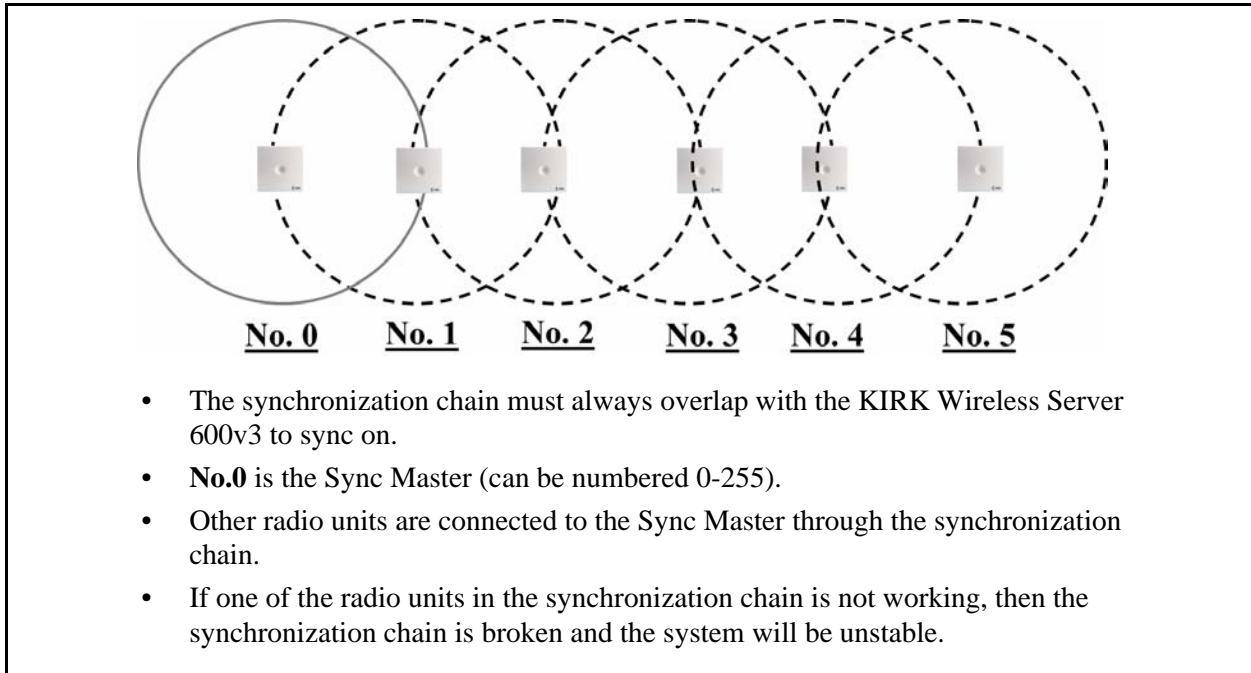
Figure 2 Synchronization Chain
